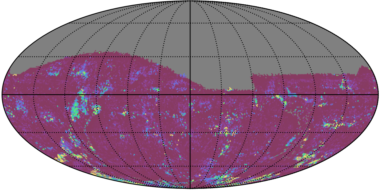
too_elab_r32_d2_ugrizy_v3.4_10yrs All sky g band: 75th Percentile Intranight Timespan
