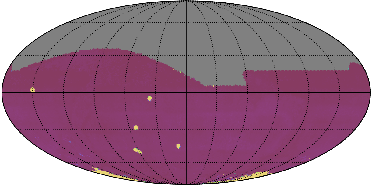
too_elab_r32_d2_ugrizy_v3.4_10yrs All sky all bands: 75th Percentile Intranight Timespan
