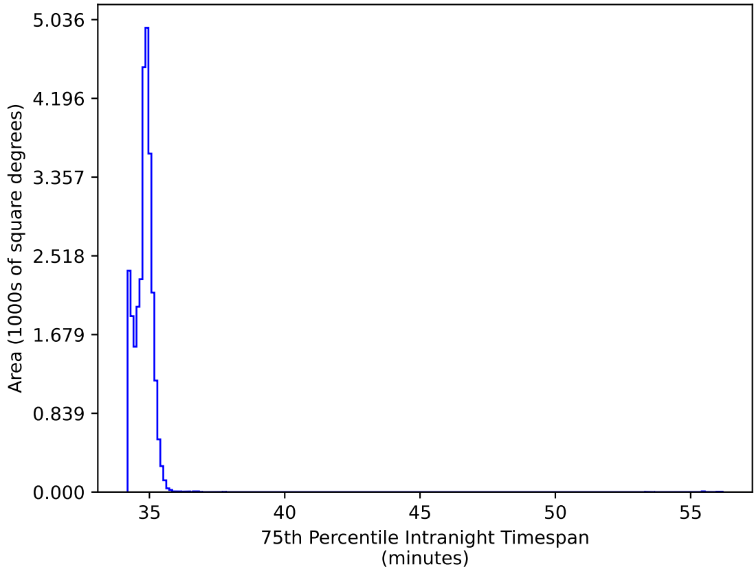
too_elab_r32_d2_ugrizy_v3.4_10yrs All sky all bands: 75th Percentile Intranight Timespan
