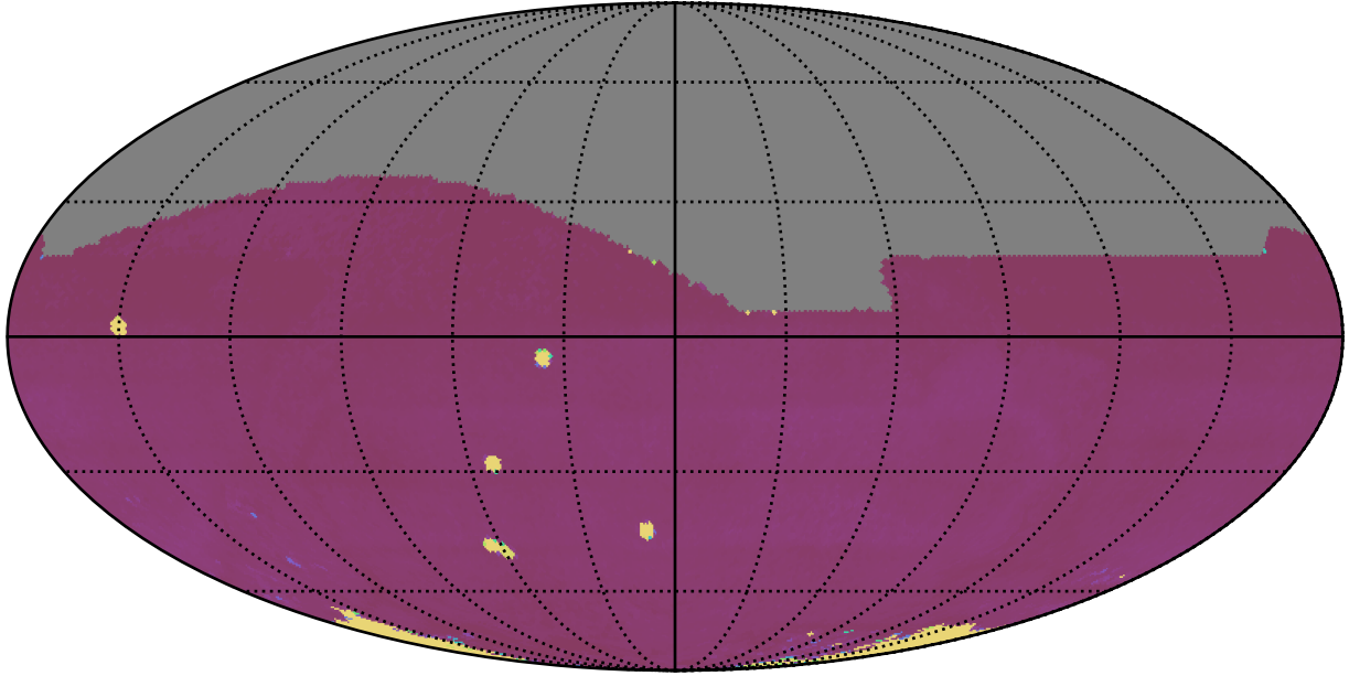
too_elab_r32_d2_ugrizy_v3.4_10yrs All sky: 75th Percentile Intranight Timespan
