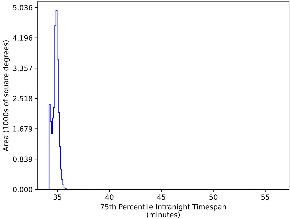
too_elab_r32_d2_ugrizy_v3.4_10yrs All sky: 75th Percentile Intranight Timespan
