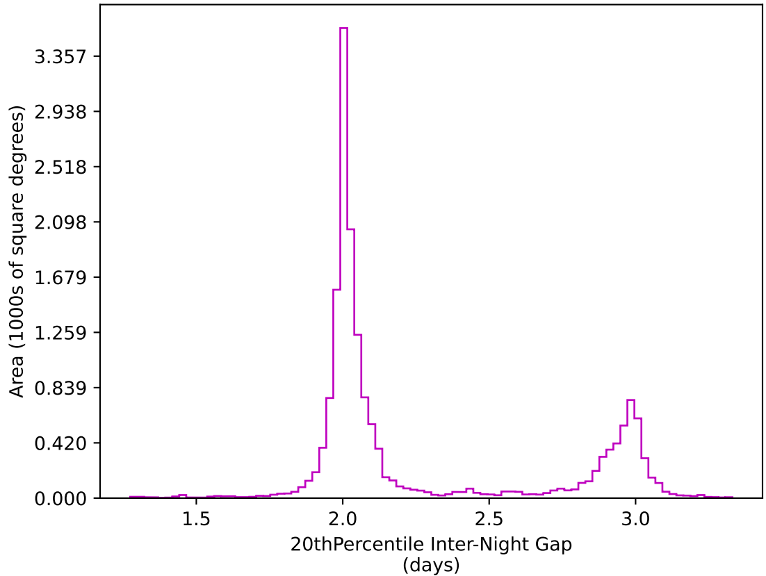
too_elab_r32_d2_ugrizy_v3.4_10yrs WFD z band: 20thPercentile Inter-Night Gap
