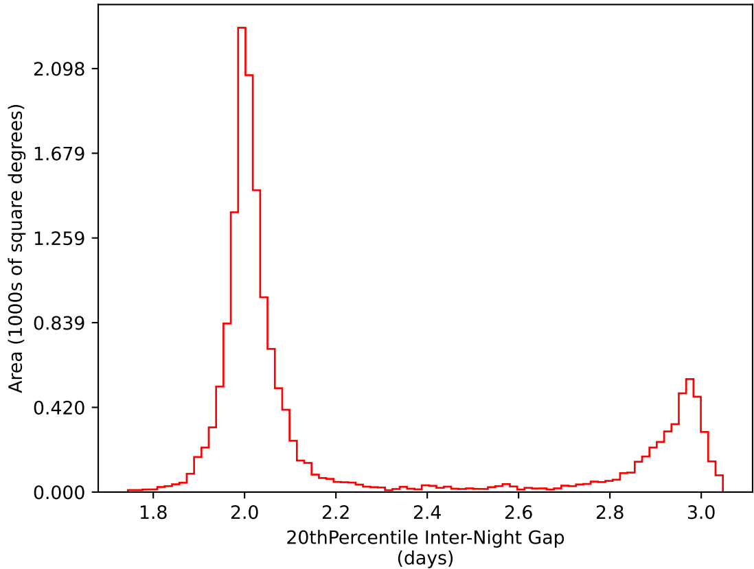
too_elab_r32_d2_ugrizy_v3.4_10yrs WFD i band: 20thPercentile Inter-Night Gap
