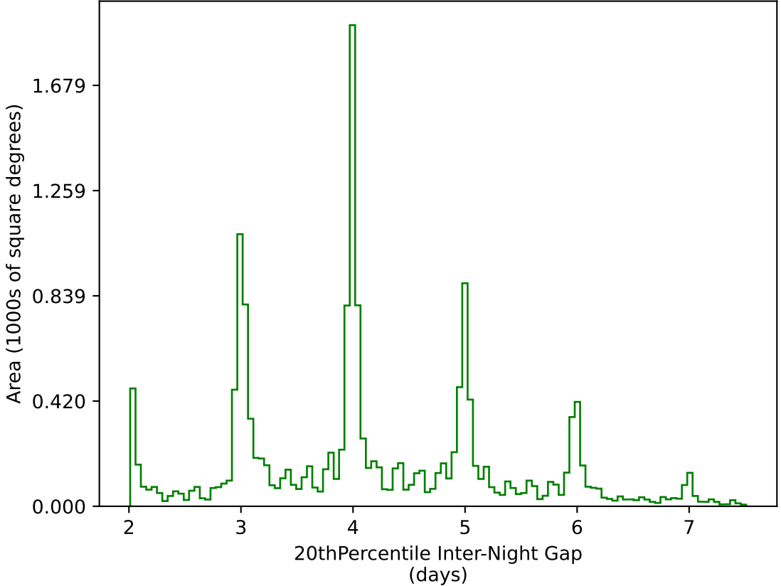
too_elab_r32_d2_ugrizy_v3.4_10yrs WFD g band: 20thPercentile Inter-Night Gap
