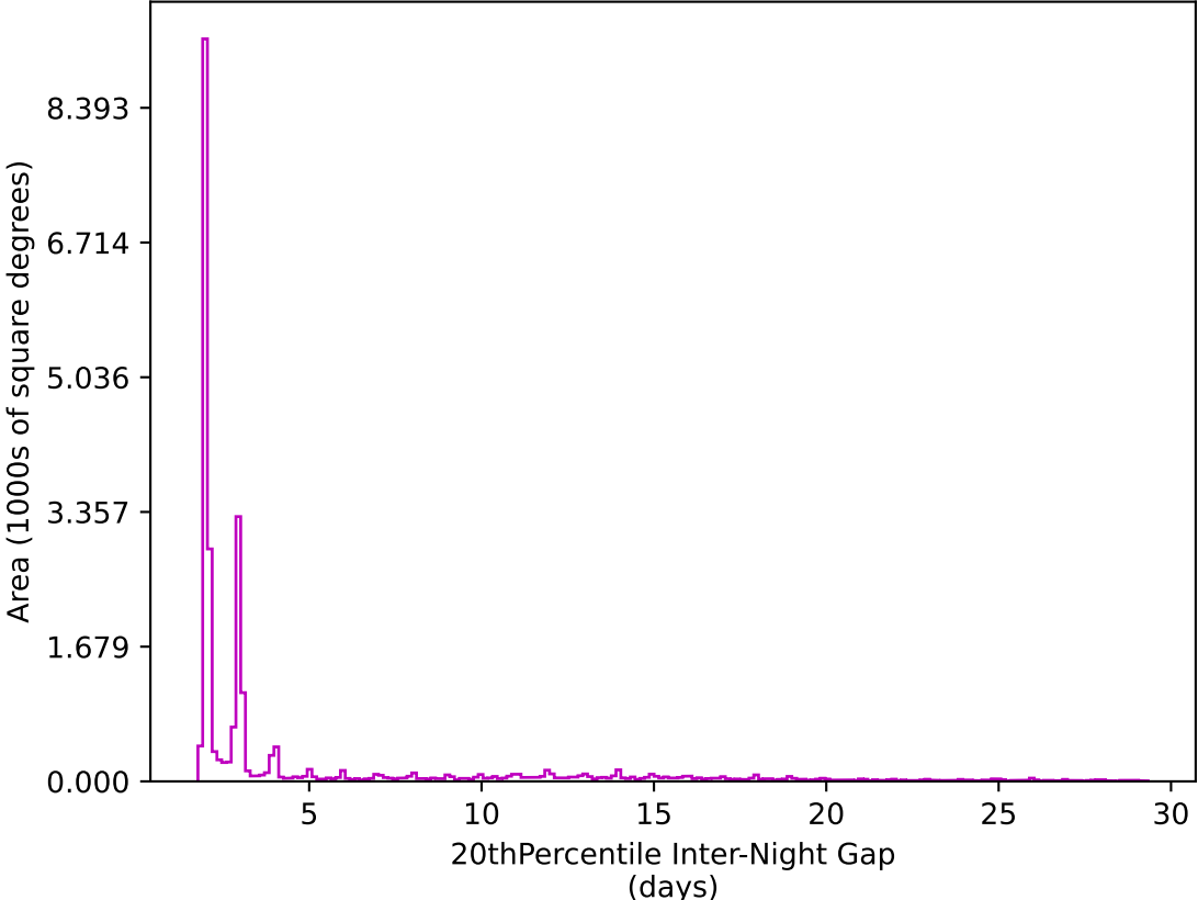
too_elab_r32_d2_ugrizy_v3.4_10yrs All sky z band: 20thPercentile Inter-Night Gap
