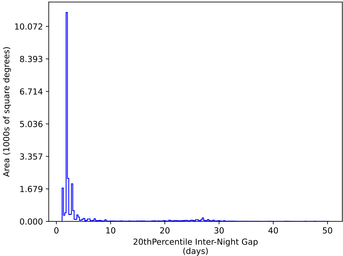
too_elab_r32_d2_ugrizy_v3.4_10yrs All sky y band: 20thPercentile Inter-Night Gap
