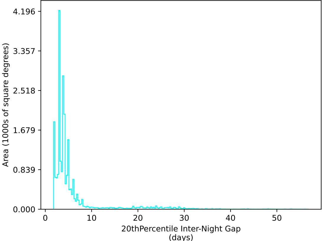
too_elab_r32_d2_ugrizy_v3.4_10yrs All sky u band: 20thPercentile Inter-Night Gap
