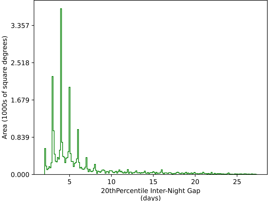
too_elab_r32_d2_ugrizy_v3.4_10yrs All sky g band: 20thPercentile Inter-Night Gap
