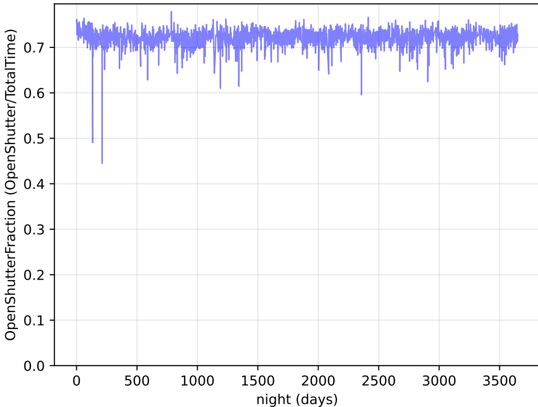
too_elab_r32_d2_ugrizy_v3.4_10yrs : OpenShutterFraction
