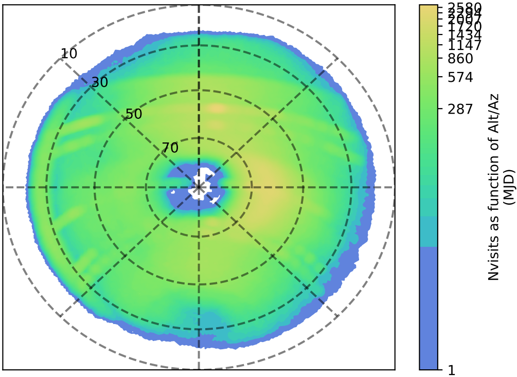
too_elab_r32_d2_ugrizy_v3.4_10yrs r: Nvisits as function of Alt/Az
