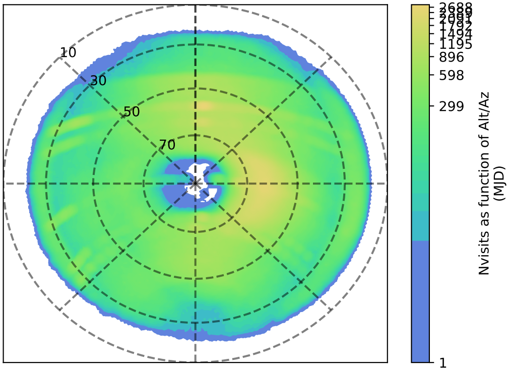
too_elab_r32_d2_ugrizy_v3.4_10yrs i: Nvisits as function of Alt/Az
