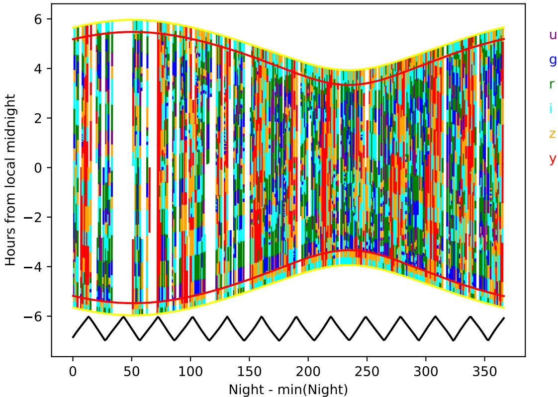
too_elab_r32_d2_ugrizy_v3.4_10yrs year 8-9: Hourglass
