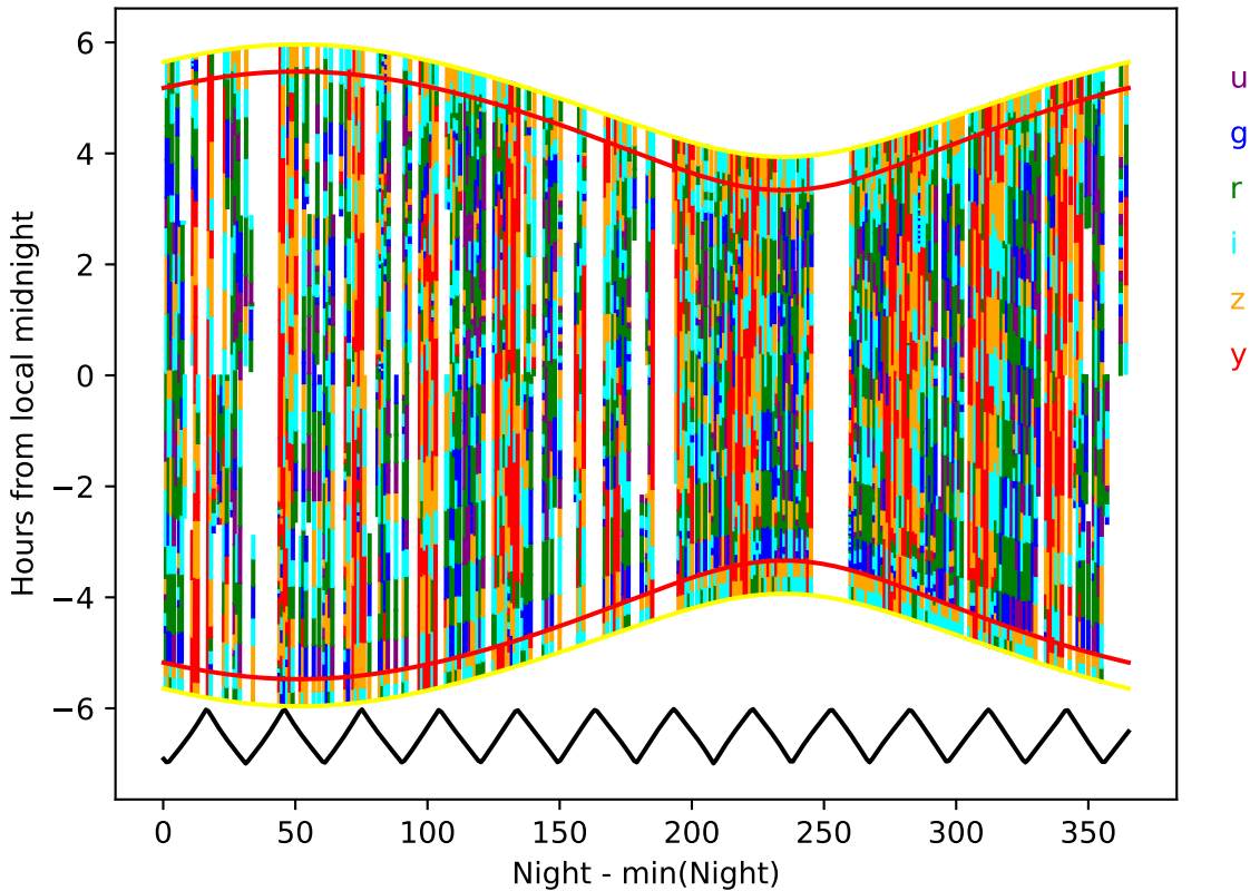
too_elab_r32_d2_ugrizy_v3.4_10yrs year 5-6: Hourglass
