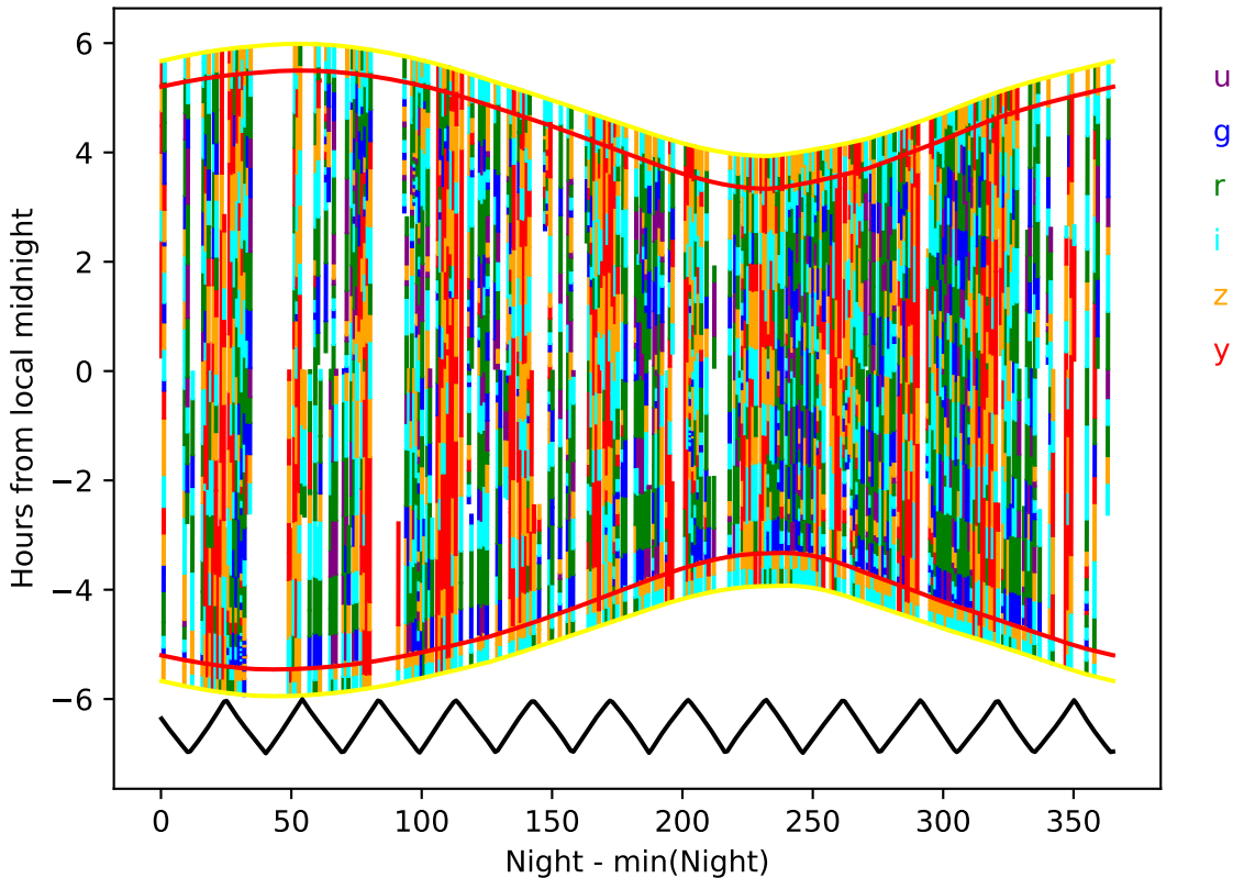
too_elab_r32_d2_ugrizy_v3.4_10yrs year 4-5: Hourglass
