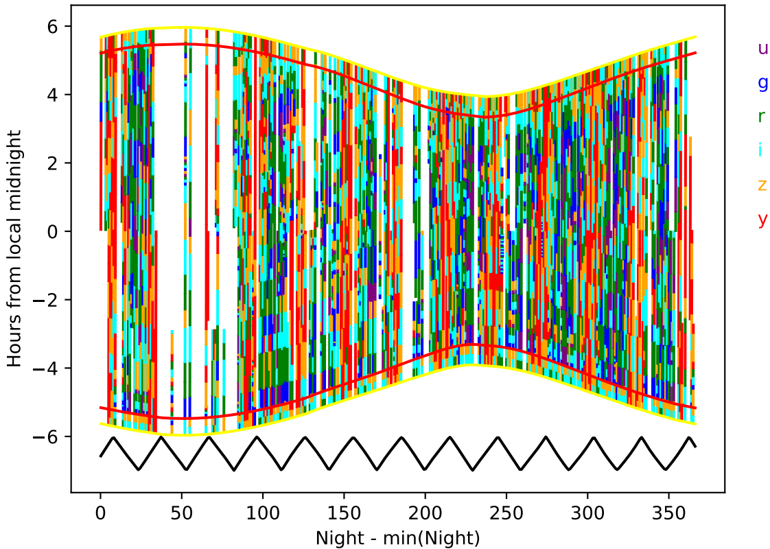
too_elab_r32_d2_ugrizy_v3.4_10yrs year 3-4: Hourglass
