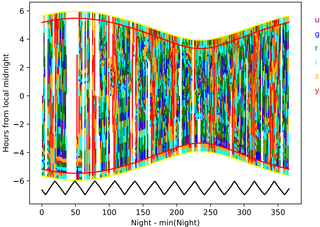
too_elab_r32_d2_ugrizy_v3.4_10yrs year 2-3: Hourglass
