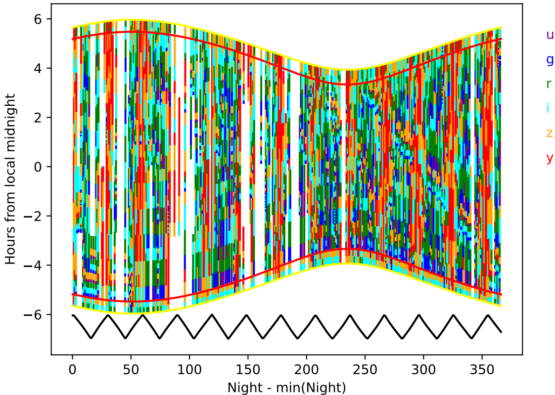
too_elab_r32_d2_ugrizy_v3.4_10yrs year 1-2: Hourglass
