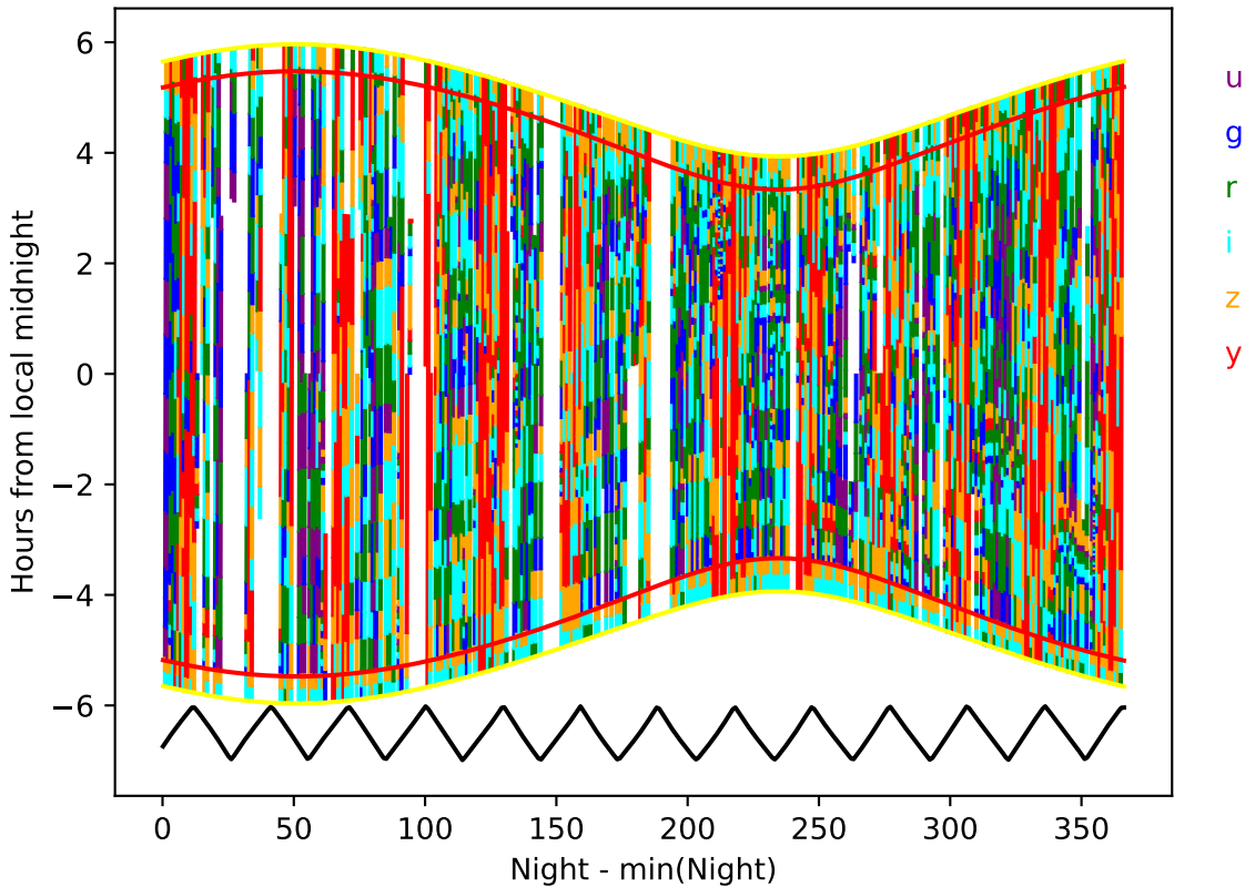
too_elab_r32_d2_ugrizy_v3.4_10yrs year 0-1: Hourglass
