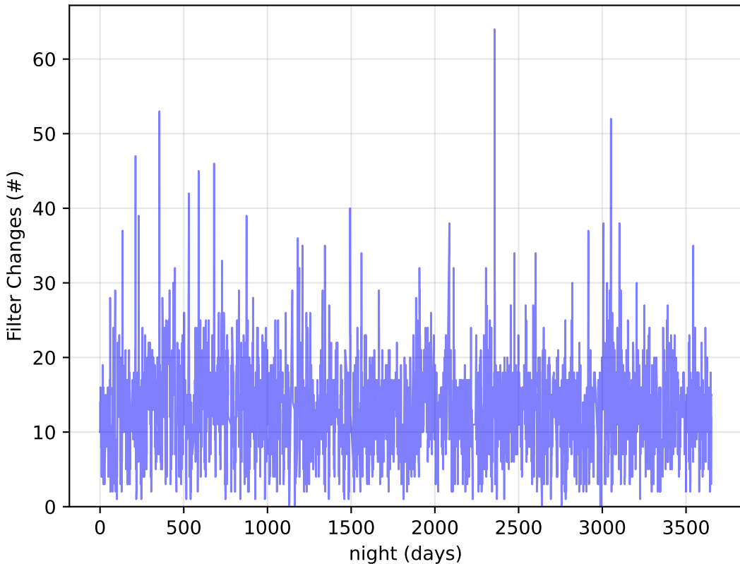
too_elab_r32_d2_ugrizy_v3.4_10yrs : Filter Changes
