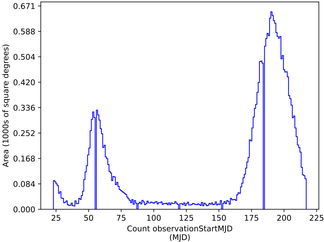
too_elab_r32_d2_ugrizy_v3.4_10yrs i: Count observationStartMJD
