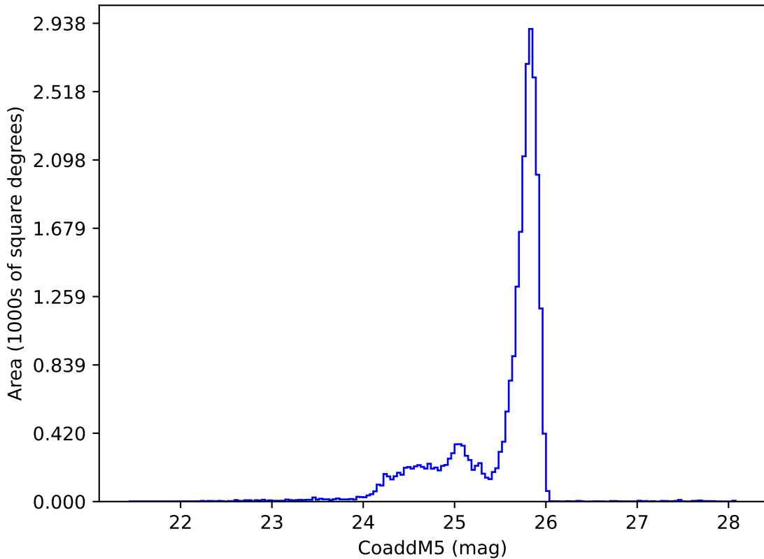
too_elab_r32_d2_ugrizy_v3.4_10yrs z: CoaddM5
