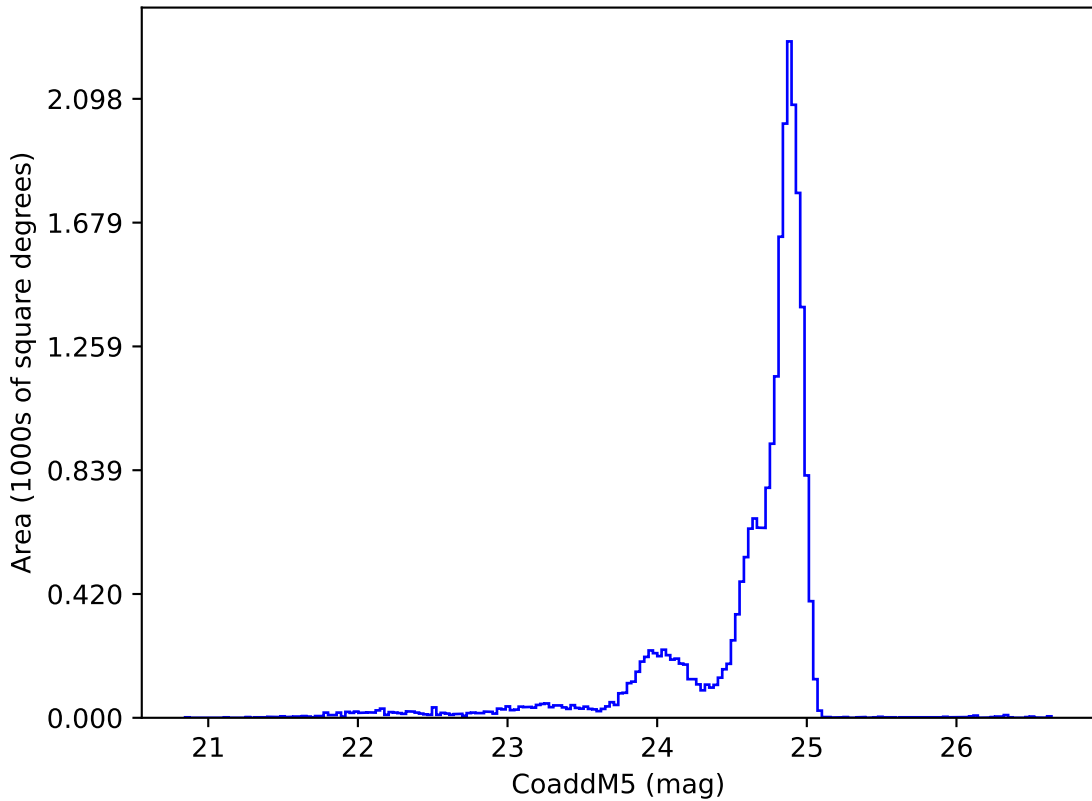
too_elab_r32_d2_ugrizy_v3.4_10yrs y: CoaddM5
