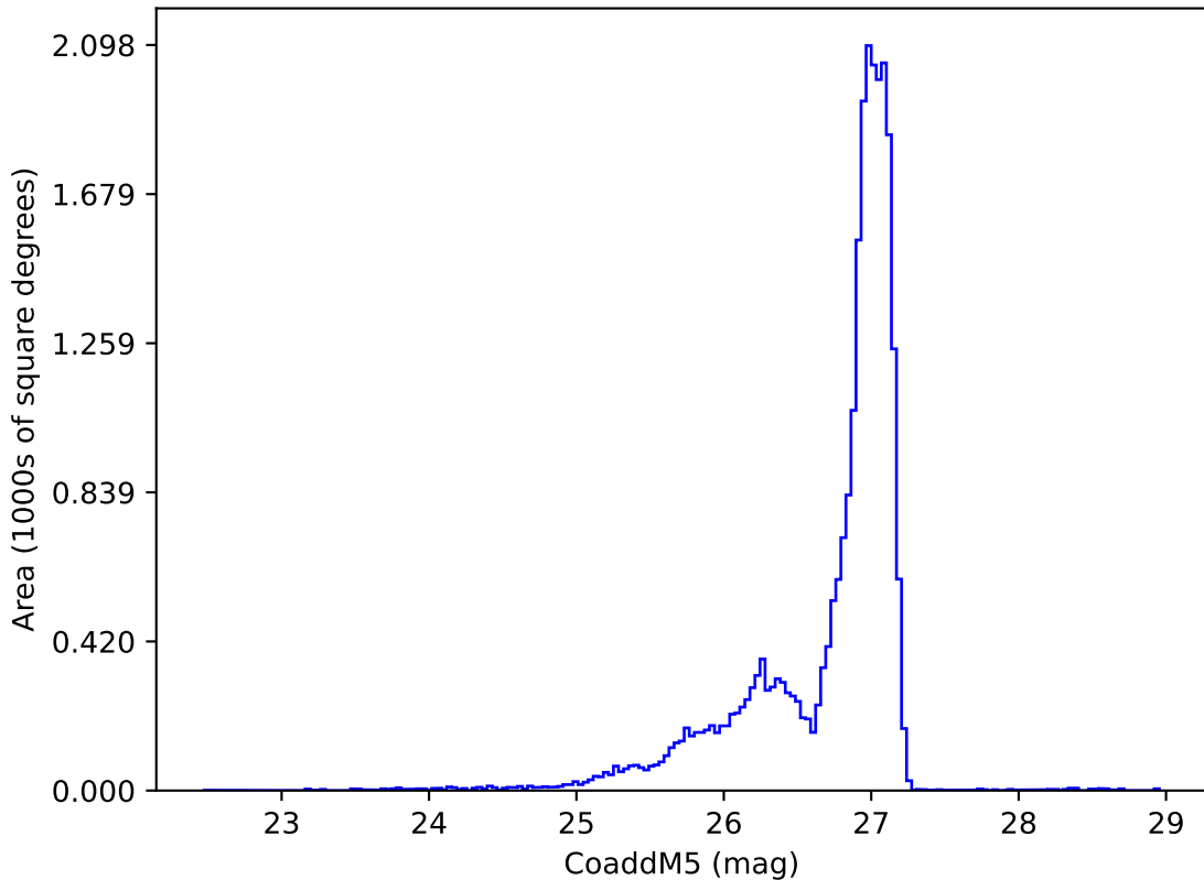
too_elab_r32_d2_ugrizy_v3.4_10yrs r: CoaddM5
