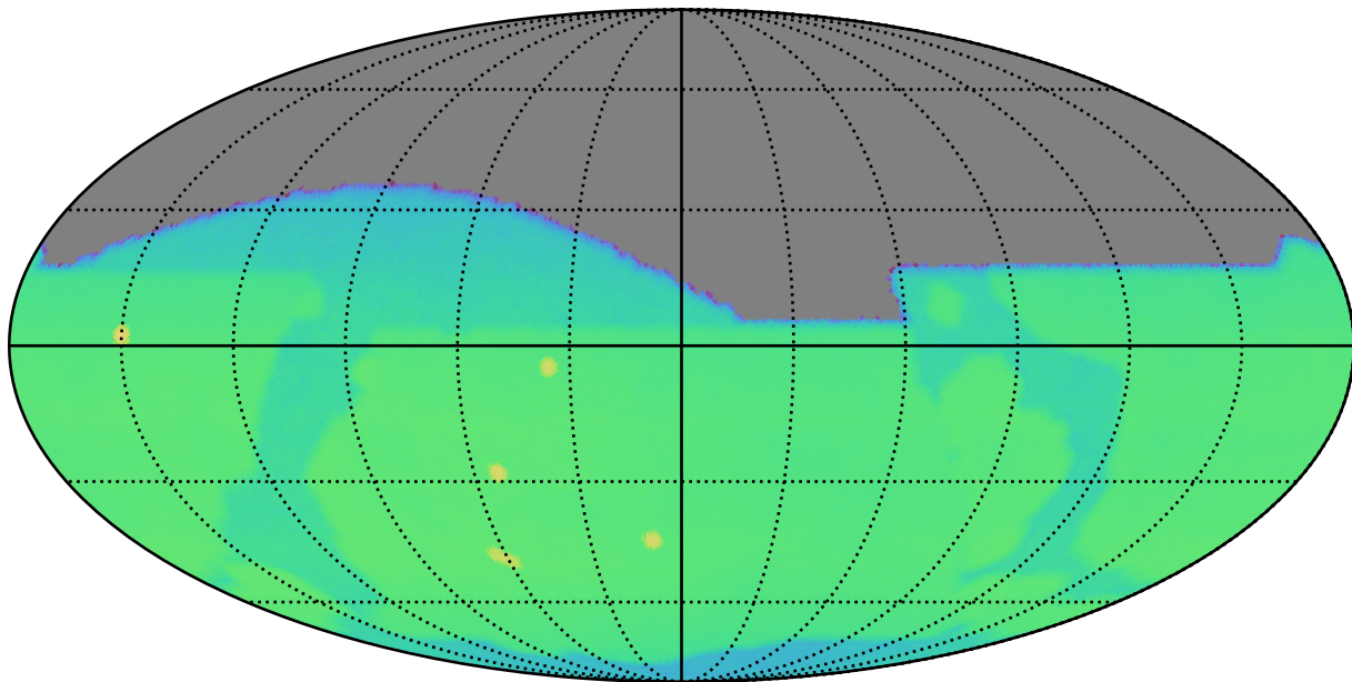
too_elab_r32_d2_ugrizy_v3.4_10yrs : CoaddM5
