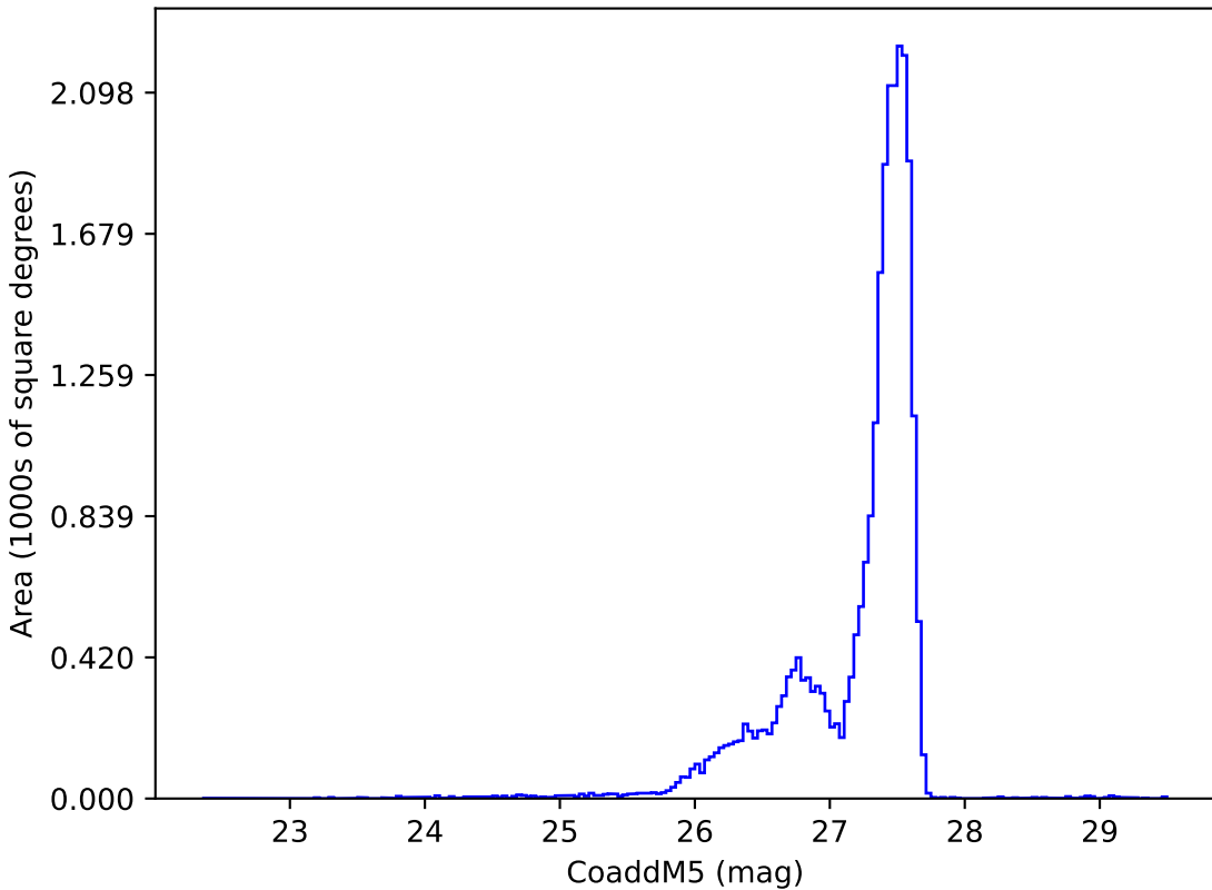
too_elab_r32_d2_ugrizy_v3.4_10yrs : CoaddM5
