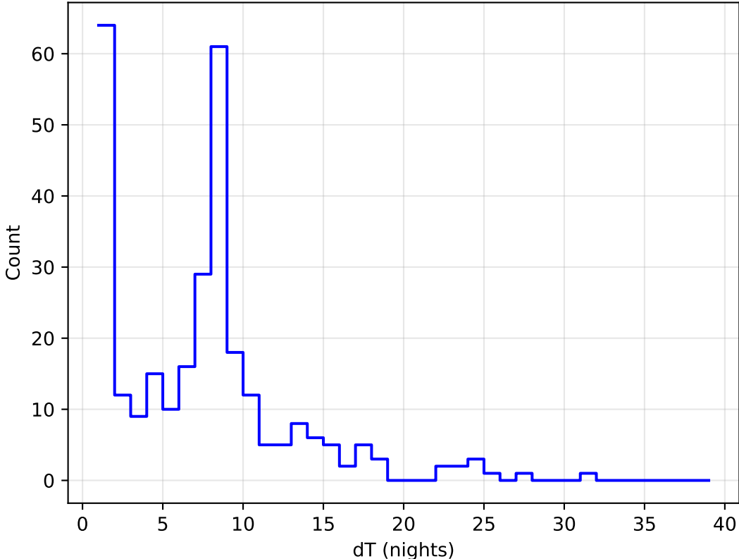
too_elab_r32_d2_ugrizy_v3.4_10yrs all bands: DD:XMM_LSS Delta Nights Histogram
