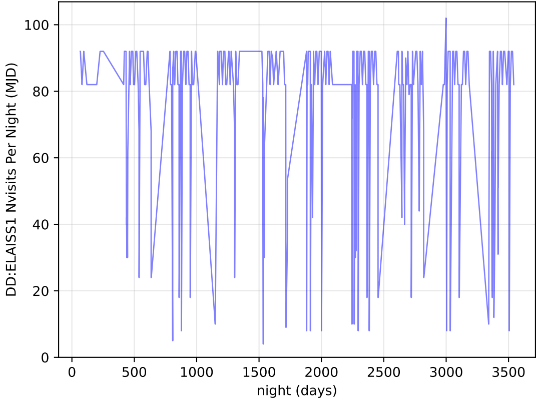
too_elab_r32_d2_ugrizy_v3.4_10yrs all bands: DD:ELAISS1 Nvisits Per Night
