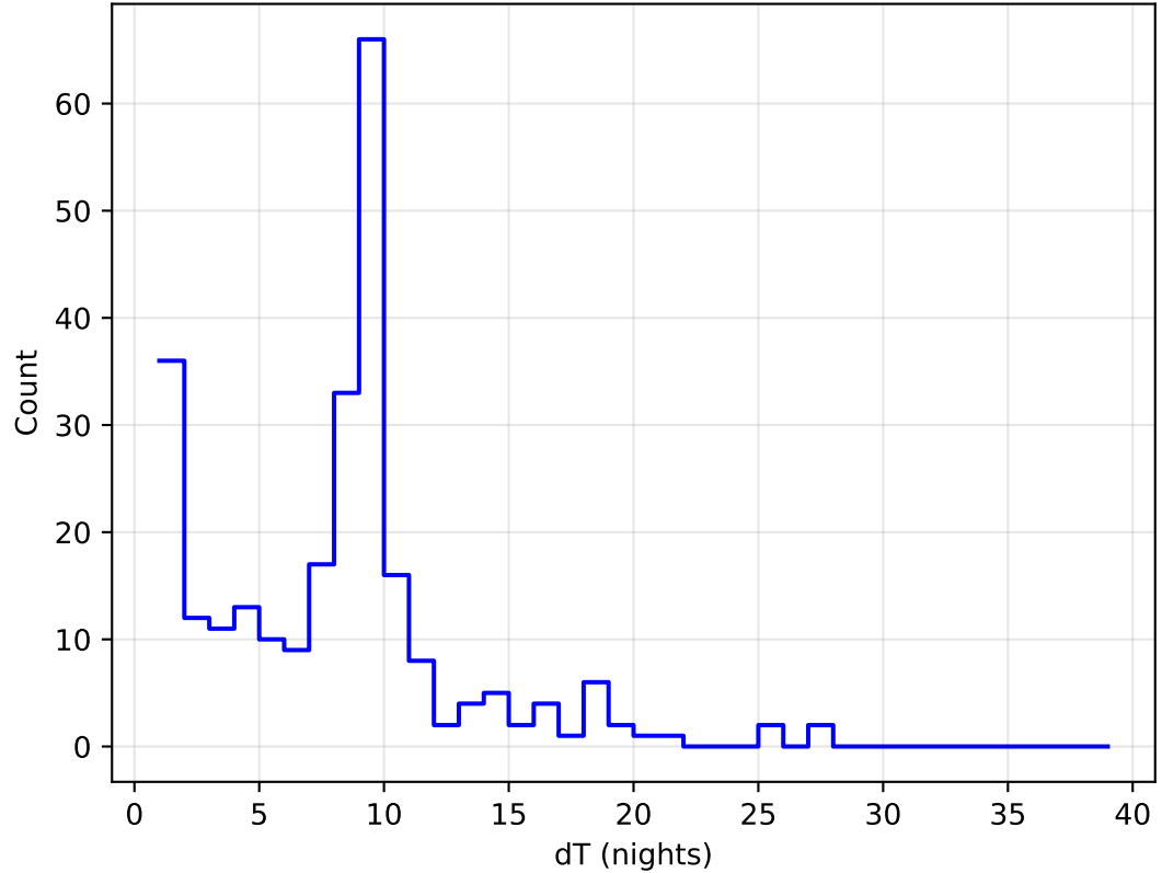
too_elab_r32_d2_ugrizy_v3.4_10yrs all bands: DD:ELAISS1 Delta Nights Histogram
