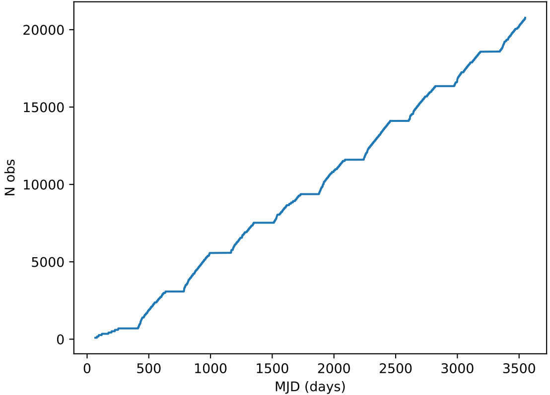
too_elab_r32_d2_ugrizy_v3.4_10yrs all bands: DD:ELAISS1 Cumulative NVisits
