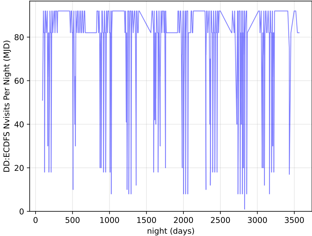
too_elab_r32_d2_ugrizy_v3.4_10yrs all bands: DD:ECDFS Nvisits Per Night
