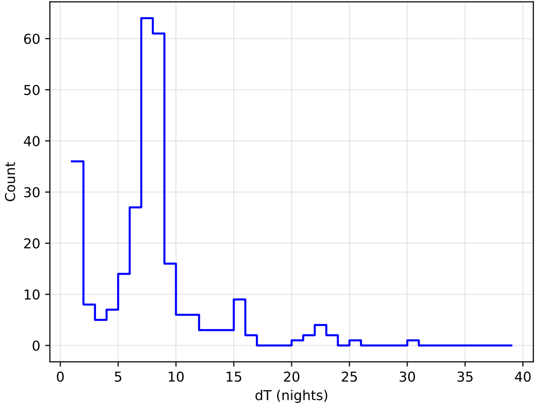
too_elab_r32_d2_ugrizy_v3.4_10yrs all bands: DD:ECDFS Delta Nights Histogram
