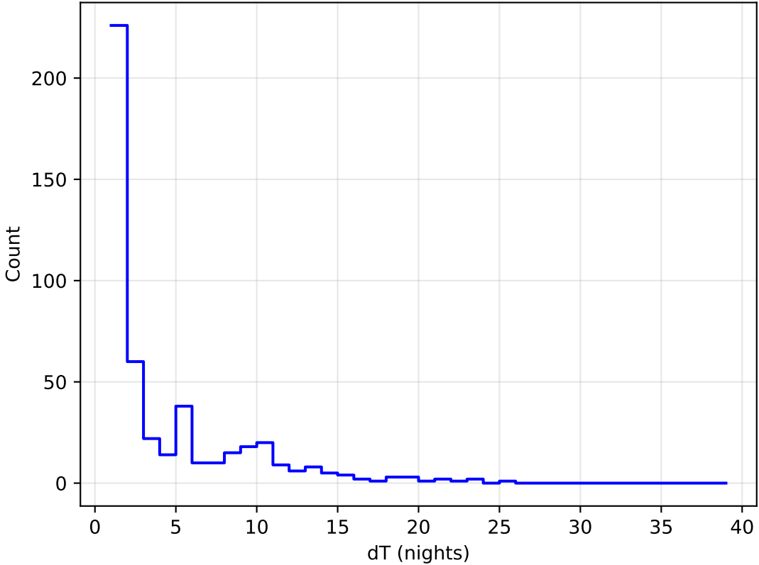
too_elab_r32_d2_ugrizy_v3.4_10yrs all bands: DD: COSMOS Delta Nights Histogram
