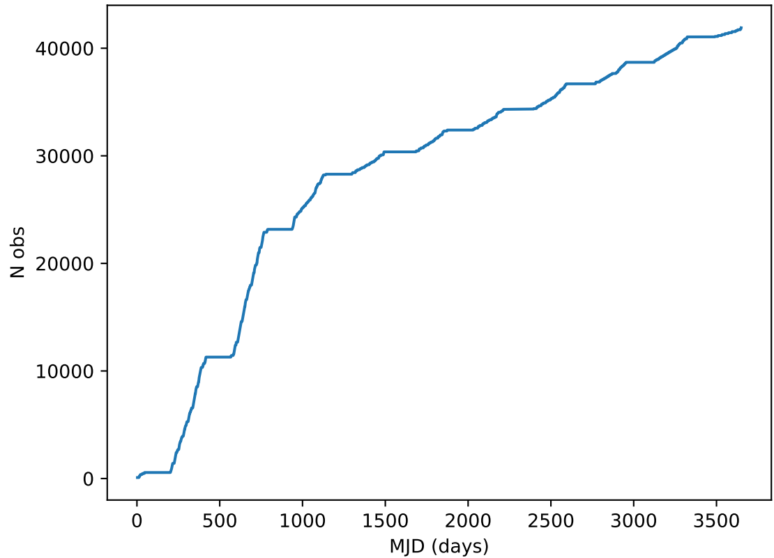
too_elab_r32_d2_ugrizy_v3.4_10yrs all bands: DD: COSMOS Cumulative NVisits
