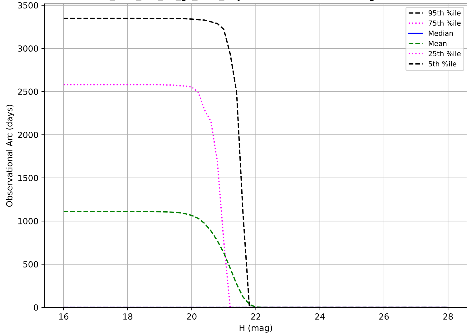
too_elab_r32_d2_gz_v3.4_10yrs: Observational Arc Length Vatra
