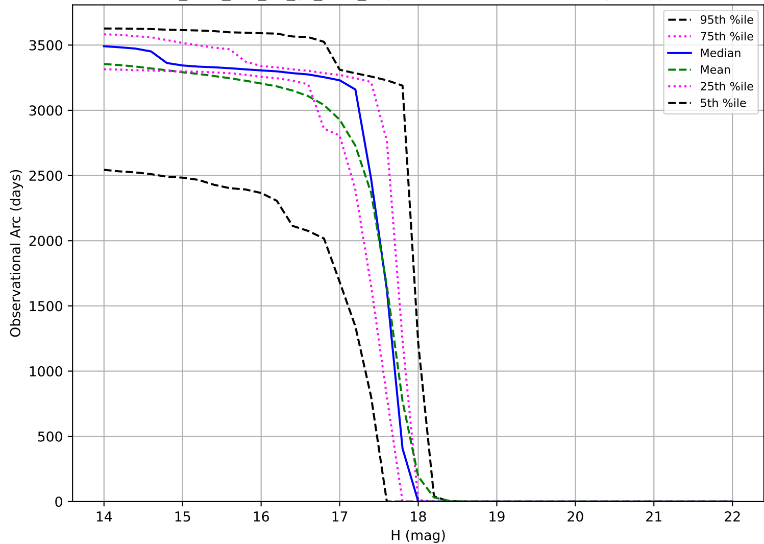
too_elab_r32_d2_gz_v3.4_10yrs: Observational Arc Length Trojan
