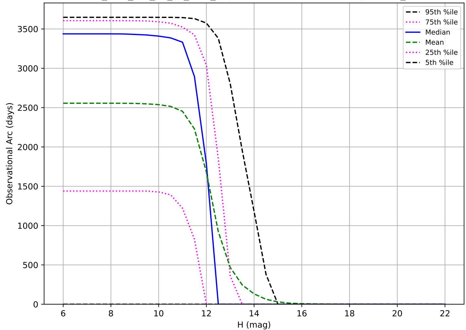
too_elab_r32_d2_gz_v3.4_10yrs: Observational Arc Length OCC_r20
