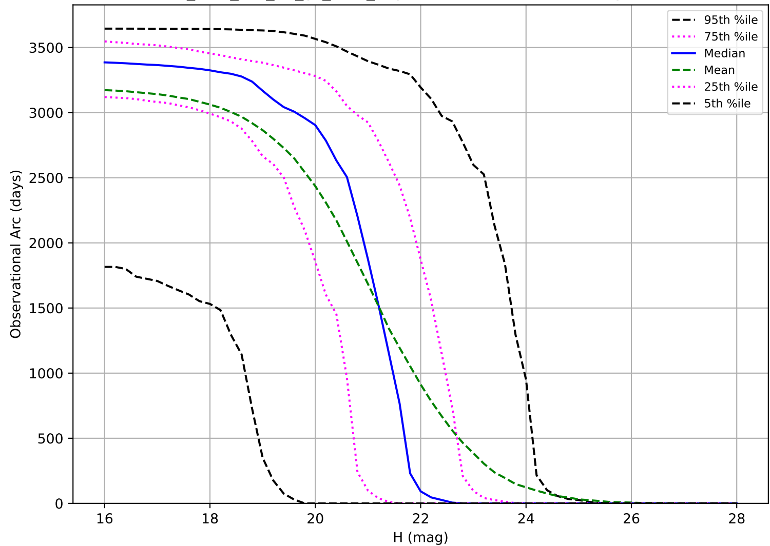
too_elab_r32_d2_gz_v3.4_10yrs: Observational Arc Length NEO
