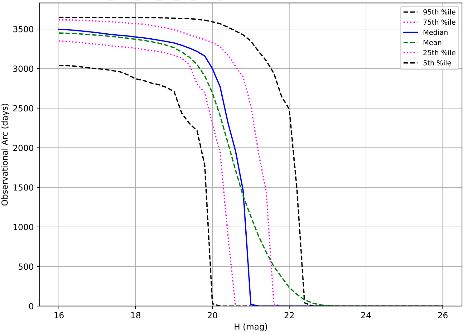
too_elab_r32_d2_gz_v3.4_10yrs: Observational Arc Length MBA
