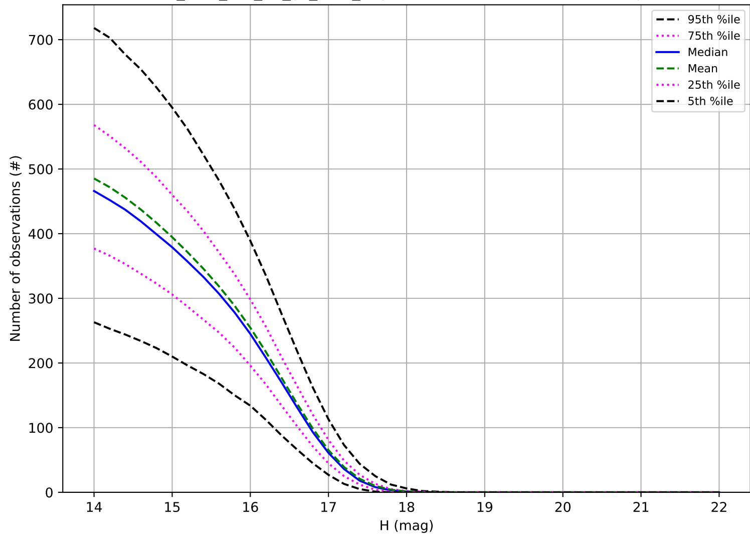
too_elab_r32_d2_gz_v3.4_10yrs: Number of observations Trojan
