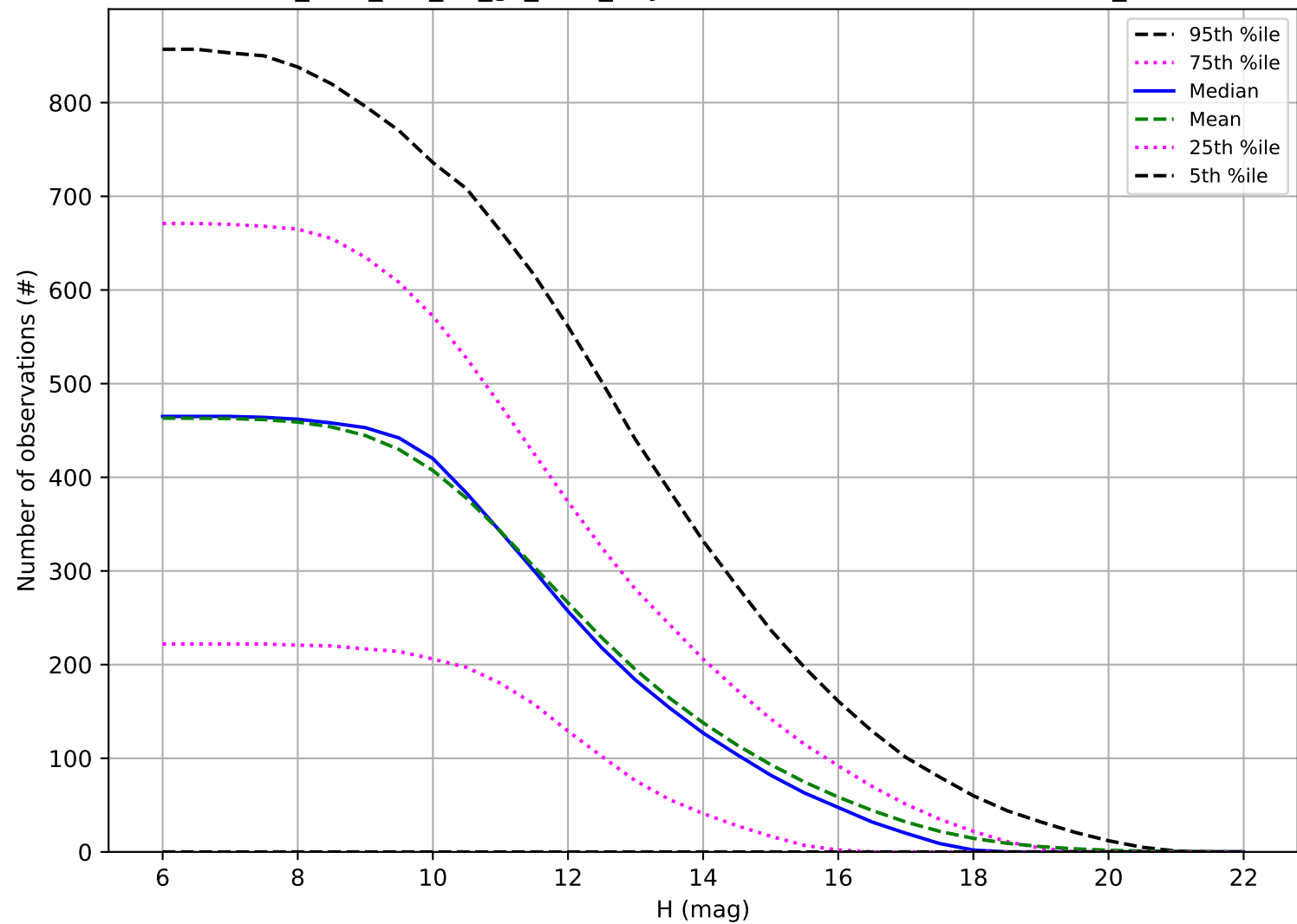
too_elab_r32_d2_gz_v3.4_10yrs: Number of observations OCC_r5
