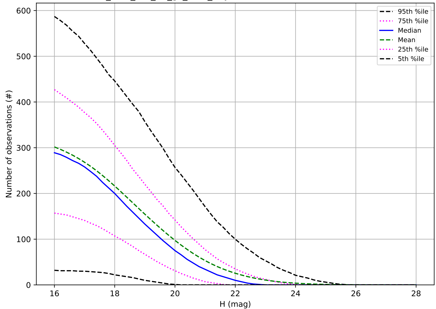
too_elab_r32_d2_gz_v3.4_10yrs: Number of observations NEO
