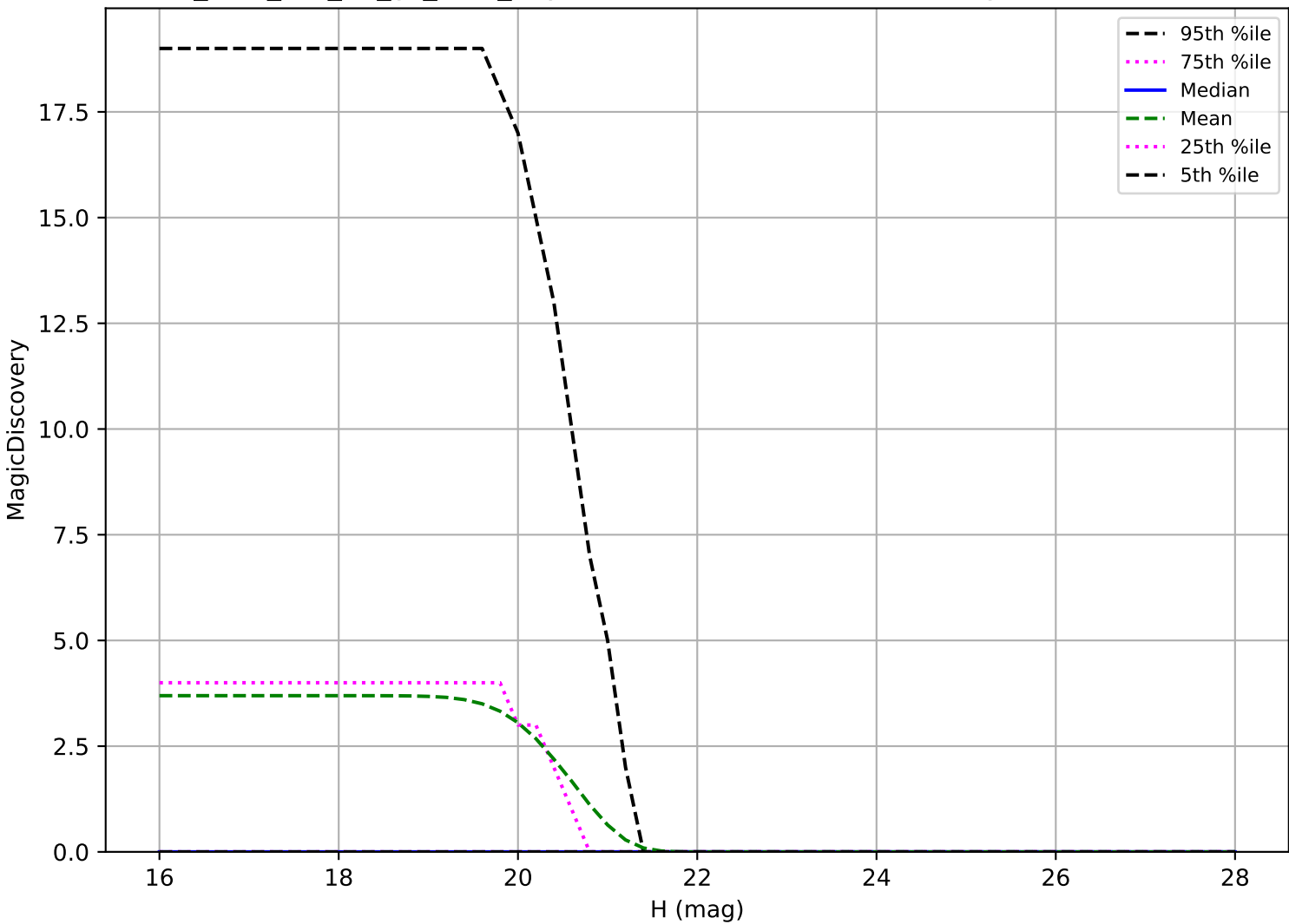
too_elab_r32_d2_gz_v3.4_10yrs: Vatira 6 detections in 60 nights detection loss
