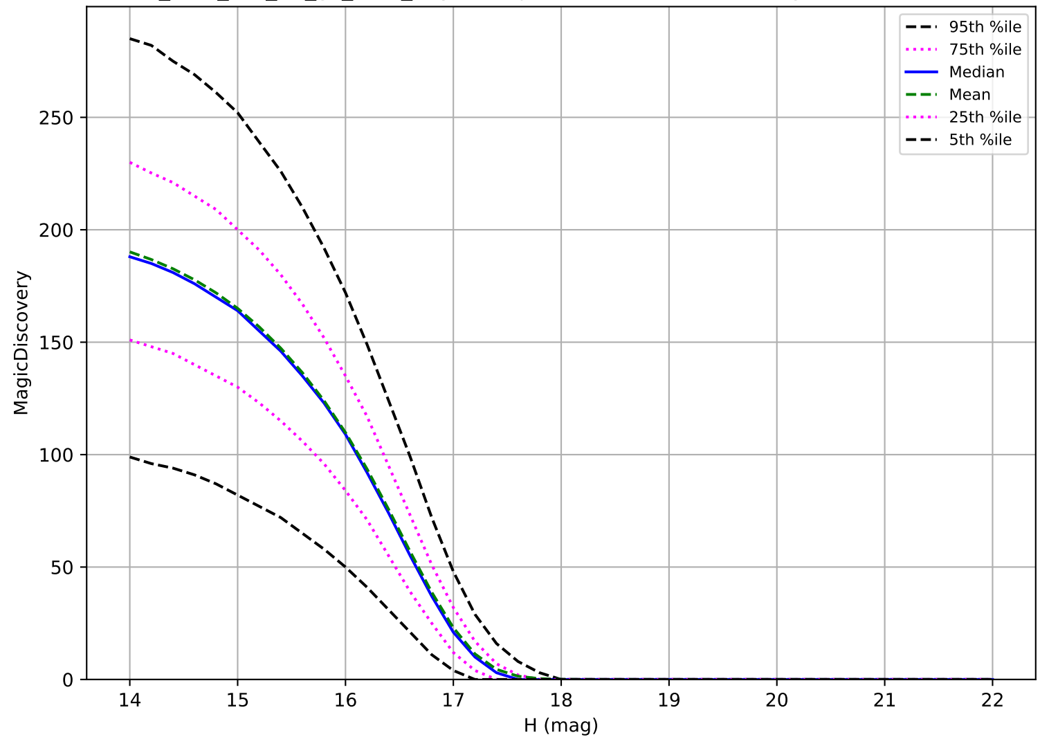
too_elab_r32_d2_gz_v3.4_10yrs: Trojan 6 detections in 60 nights detection loss
