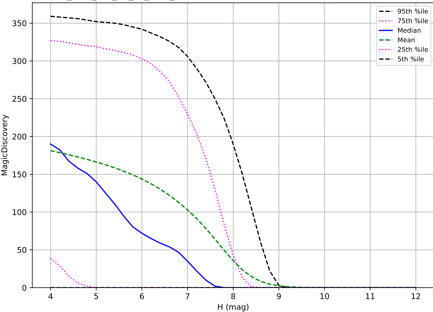
too_elab_r32_d2_gz_v3.4_10yrs: TNO 6 detections in 60 nights detection loss
