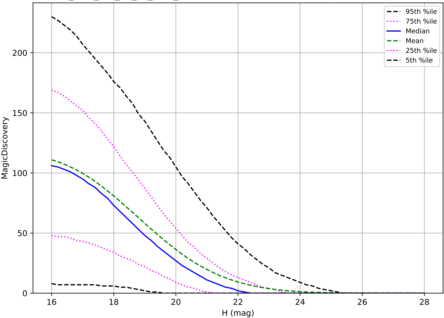
too_elab_r32_d2_gz_v3.4_10yrs: PHA 6 detections in 60 nights detection loss
