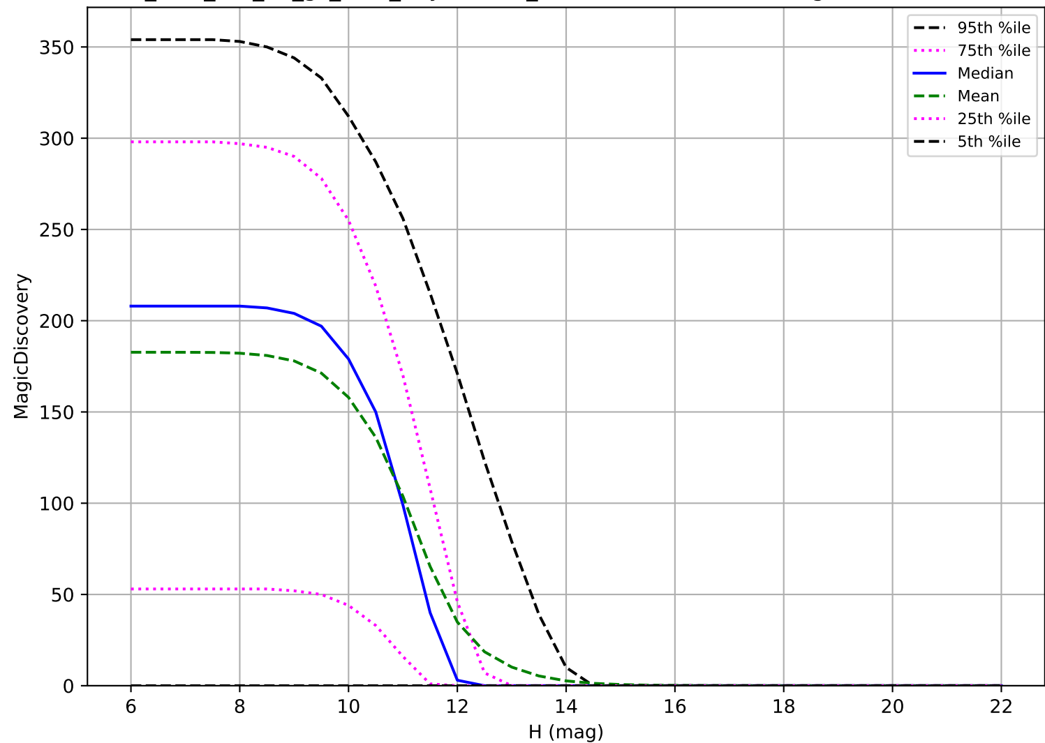
too_elab_r32_d2_gz_v3.4_10yrs: OCC_r20 6 detections in 60 nights detection loss
